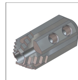
Special Drill Head (3D)
